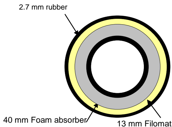
Sound Insulation Construction for tested object.
