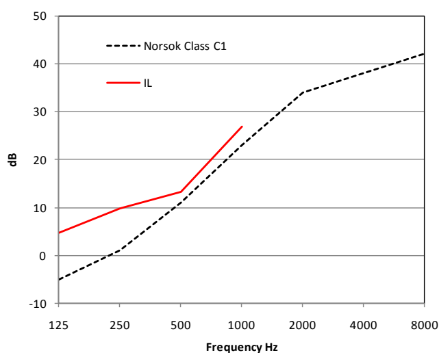
Sound Insulation Construction for tested object.
